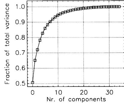
Fig. 7. Feature vectors are expanded in the eigenvectors of the covariance matrix of the available data.
